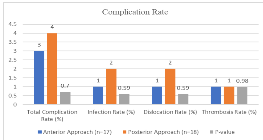
Figure 1: Complication Rates
